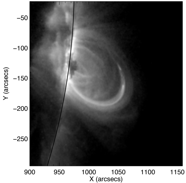
TRACE 195 18-Dec-2006 01:28:43.000 UT
