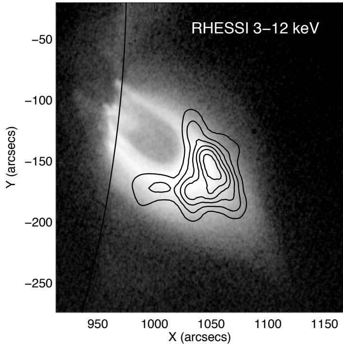
XRT C_poly 17-Dec-2006 18:22:44.979 UT
